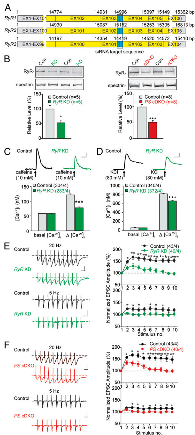
Fig. 5. Knockdown of RyR expression mimics the impaired calcium homeostasis and presynaptic function in PS cDKO neurons. (A) Schematic diagram showing the location of the shRNA targeting sequence for all three isoforms of RyR. (B) Comparison of RyR protein levels in RyR KD and PS cDKO cultures. (Left) Reduced RyR protein levels in hippocampal cultures 4 d after the lentivirus containing the shRNA sequence targeting all three isoforms of RyR is introduced to the hippocampal cultures. (Right) Reduced RyR protein levels in PS cDKO cultures. All samples are collected at DIV14. (C) Caffeine-induced calcium response is reduced in RyR KD neurons. (Upper) Representative traces of caffeine (10 mM)-induced Ca 2+ responses. (Scale bar: 5 s, 25 nM). (Lower) Summarized amplitude of caffeine-induced Ca 2+ responses in control and RyR KD neurons. (D) High potassium-induced Ca 2+ response is reduced in RyR KD neurons. (Upper) Representative traces of KCl (80 mM)-induced Ca 2+ responses.
